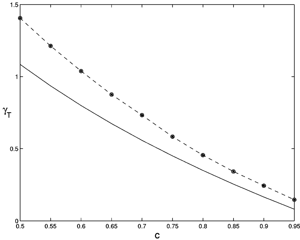
FIG. 19. The typical smoothness of the synchronization manifold as a function of the coupling strength c . The solid line is obtained from the theoretical prediction, while the dashed line is obtained from the wavelet transform. For any finite resolution level, the wavelet method provides an upper bound for \gamma_t which is consistent with the observed numerical overestimate.
