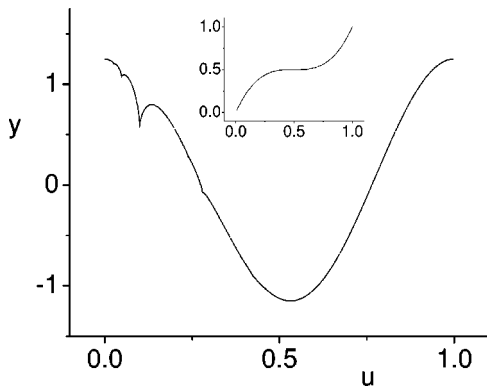
FIG. 6. Cusped case with s=0 and c=0.2 . The inset shows the shape of \omega . We set \lambda=0.2 and \alpha=0.3 , for which h_d=-0.90 and |h_d|<|h_r| . Cusps occur at the forward iterates of the critical point at u=1/2 and decrease in size due to the cumulative effect of the transverse contraction.
